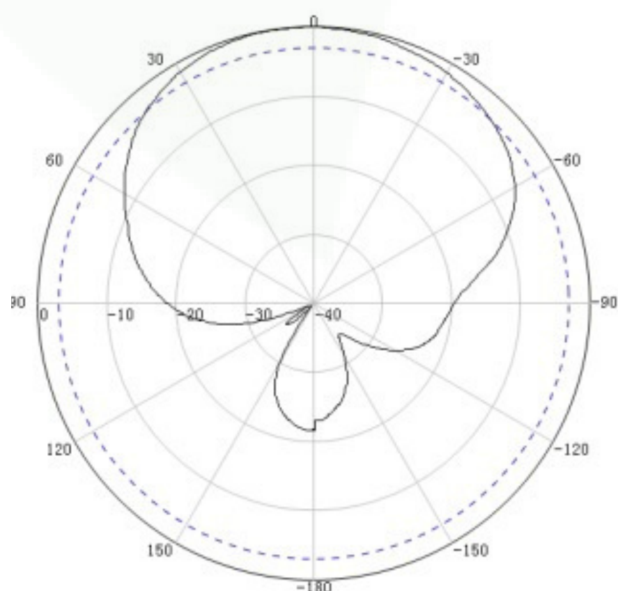
Horizontal Pattern
