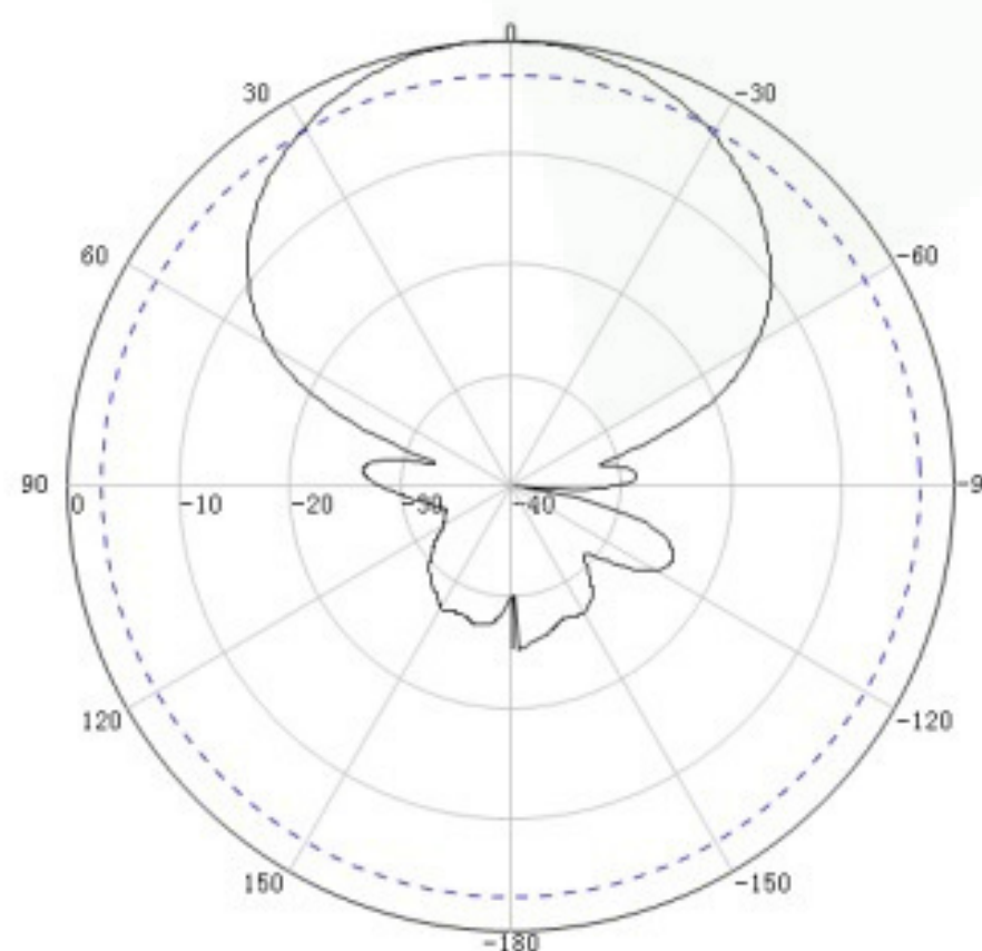
Vertical Pattern
